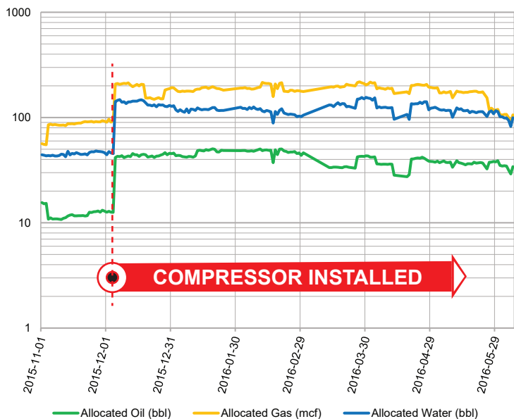
Oil well optimization with Gaspro casing gas compressor package 13-08-078-21W5.00
